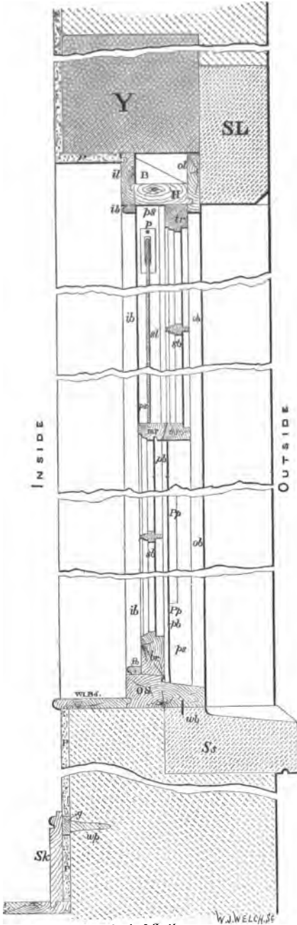
Vertical Section. (1/2) Fig. 317.
